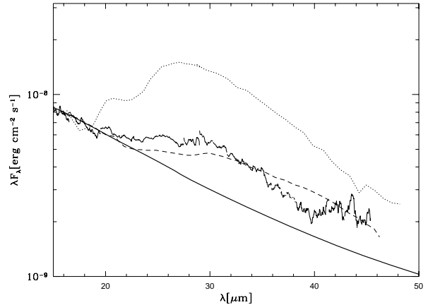
Fig. 3. Comparison of the 30 micron band in IRAS 03313+6058 (thin solid line) with the post-AGB object IRAS 22272+5435 (dotted line) and AGB star AFGL 3068 (dashed line). The modeling continuum spectrum at this band to IRAS 03313+6058 is represented by the thick solid line which lies below the emission features.
